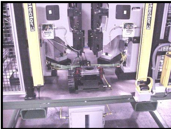
Close up shot of operator load area with light curtains.
