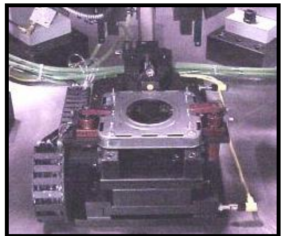
Close up shot of two (2) position slide and part presence sensors.
