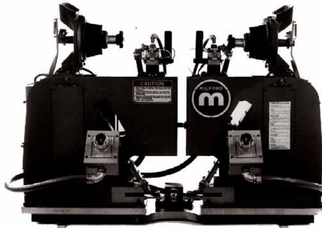
Two horizontals set up for simultaneous, high production riveting from opposite sides.
